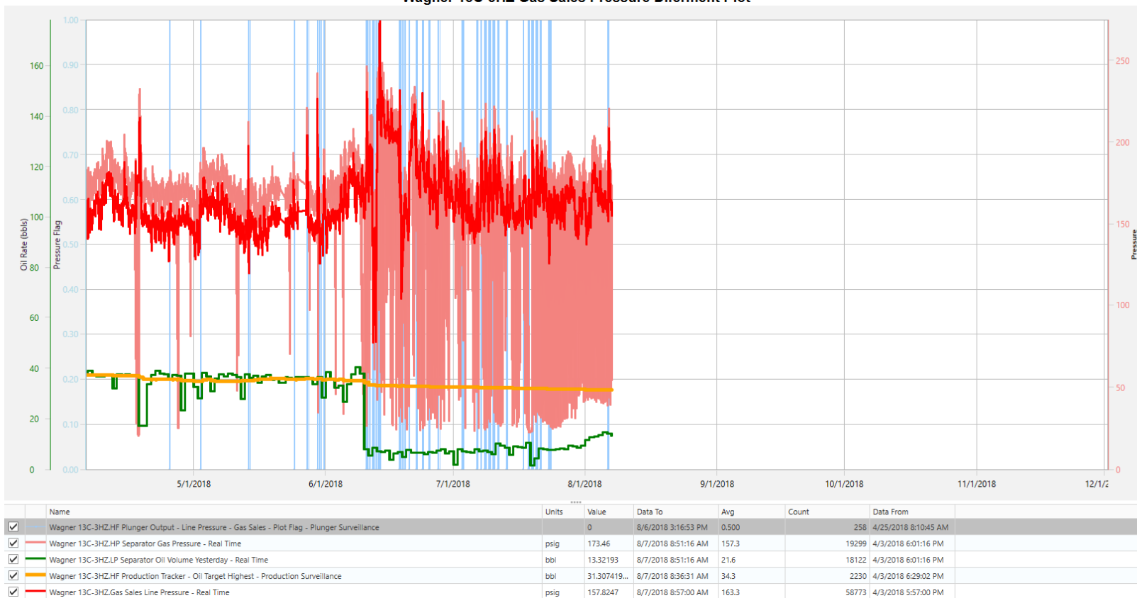
Wagner 13C-3HZ Gas Sales Pressure Diferment Plot
