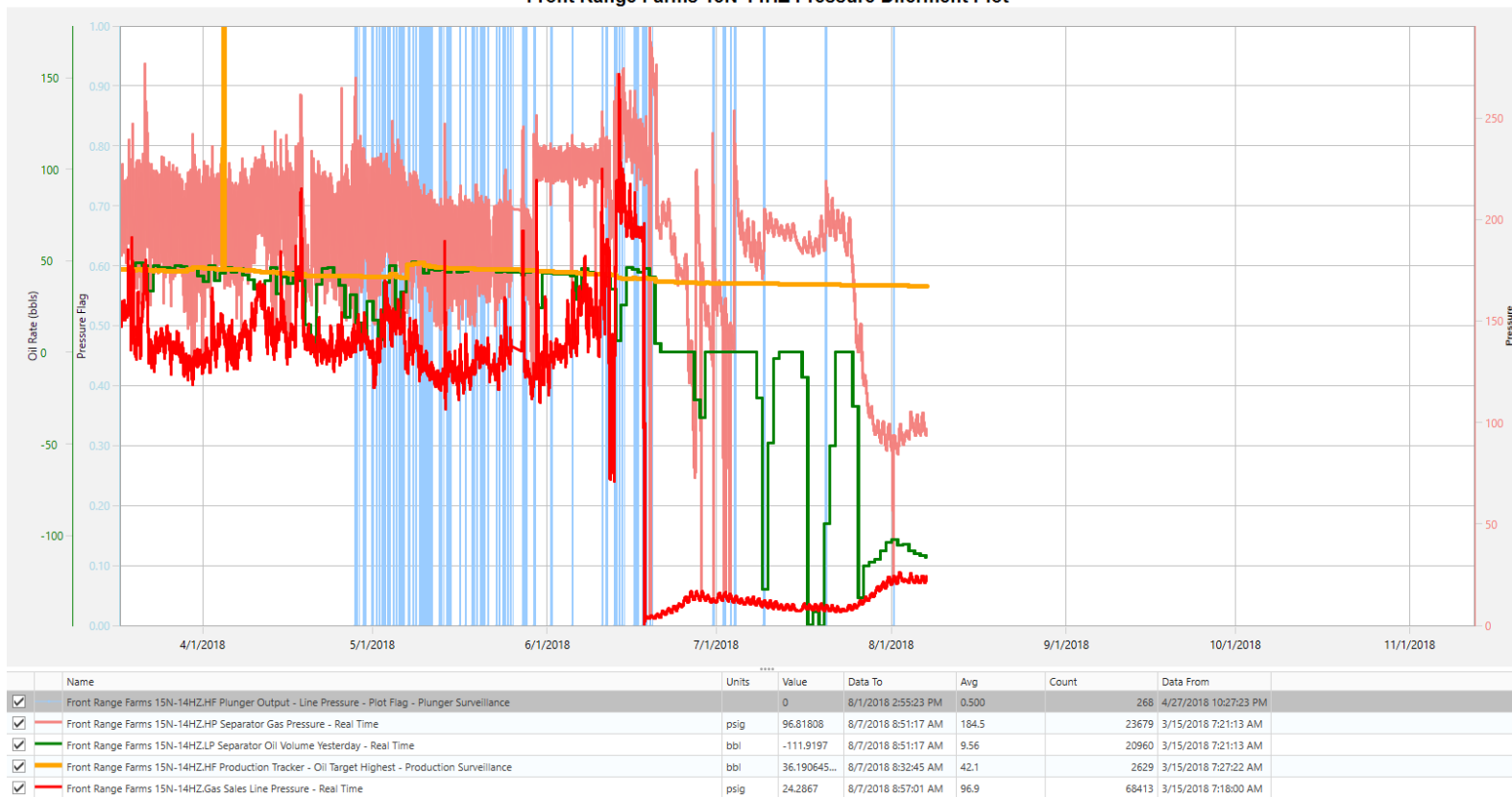
Front Range Farms 15N-14HZ Pressure Diferment Plot
